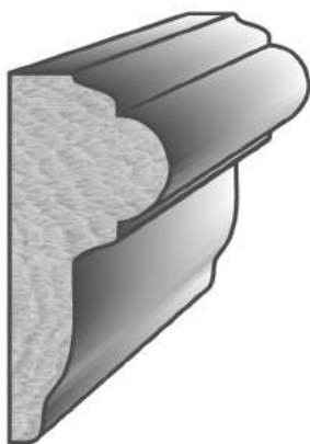
U759 Chair Rail \frac{3}{4}'' \times 1\frac{3}{4}''
