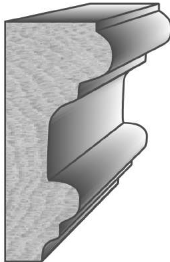
U751 Chair Rail
