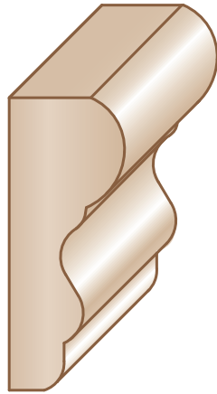
M600 Chair Rail \frac{5}{8}'' \times 1 \frac{5}{8}''
