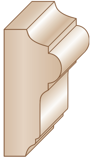
U782 Chair Rail 1 1/4" x 2 3/4"
