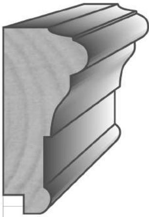
1/4" Rabbetted U762 Chair Rail 7/8" x 2"
