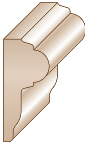
M608 Chair Rail \frac{3}{4}'' \times 1 \frac{3}{4}''
